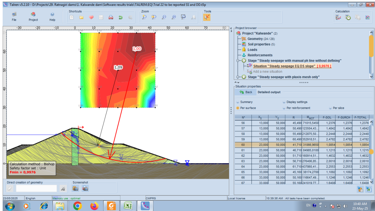
Figure 5.8 Search for critical slip circle with lowest Factor of Safety
