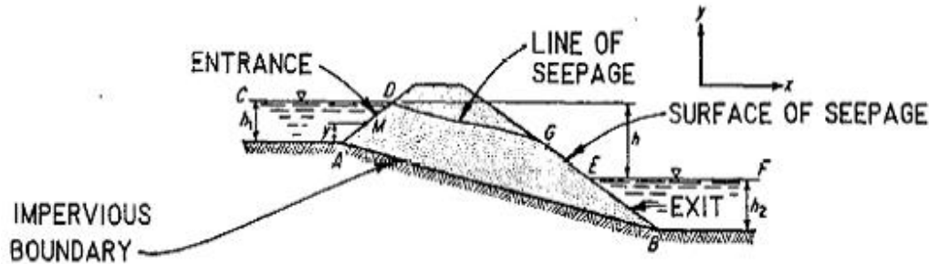
Figure 4.3 Unconfined flow through earthen dam
