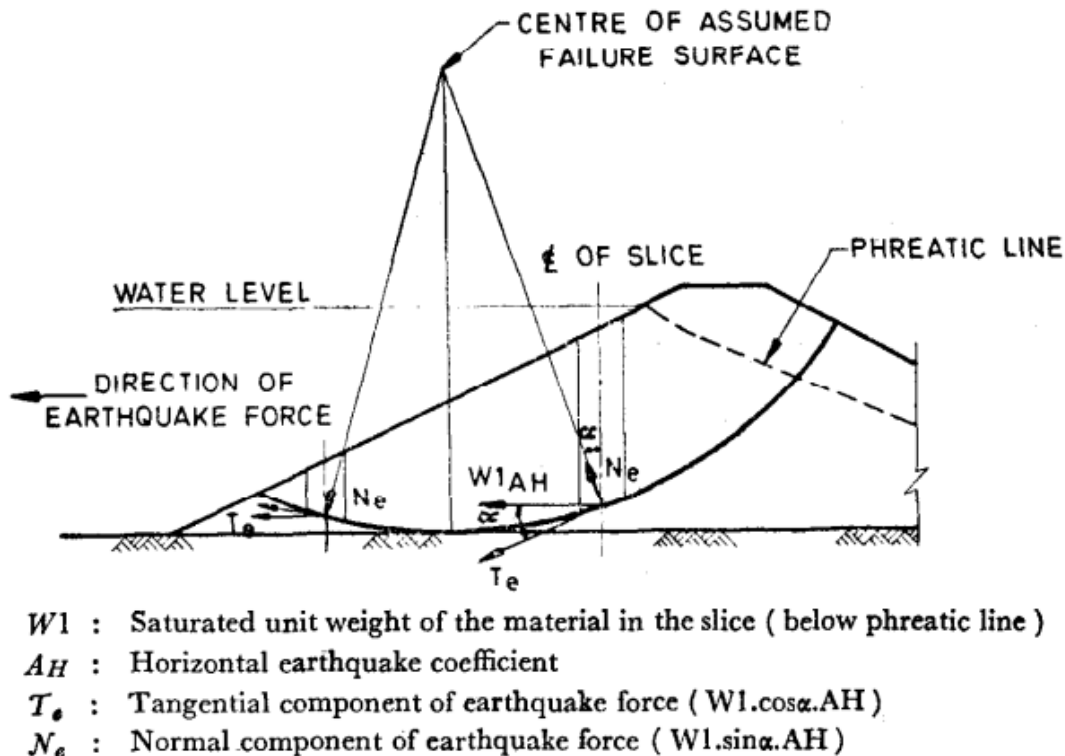
Figure 6.4 Pseudo-static limit equilibrium slope stability method
