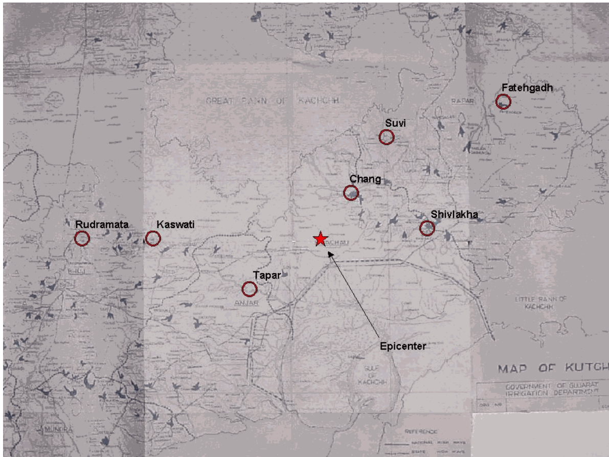
Figure 6.1 Location of earthen dams damaged during Bhuj earthquake
